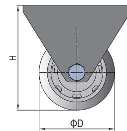
Castor-Plate-Fixed-Heavy
