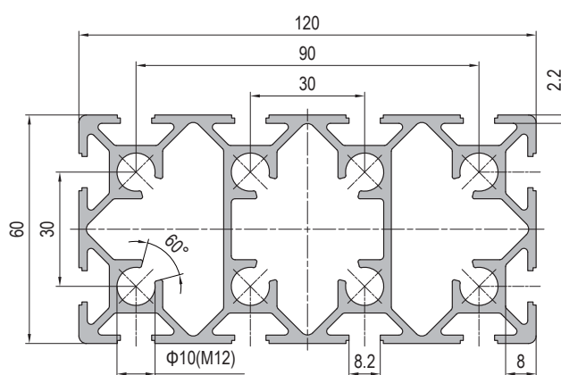
60x120 12 slots
