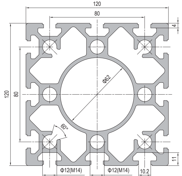
120x120 12 slots
