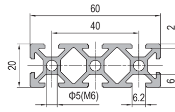
20x60 8 slots
